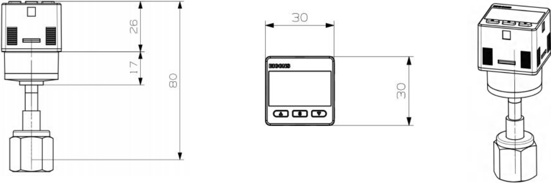
Top digital display 9/16-18UNF female thread
