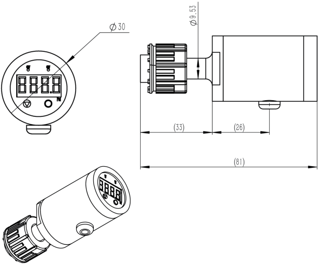
3/8" Flared
