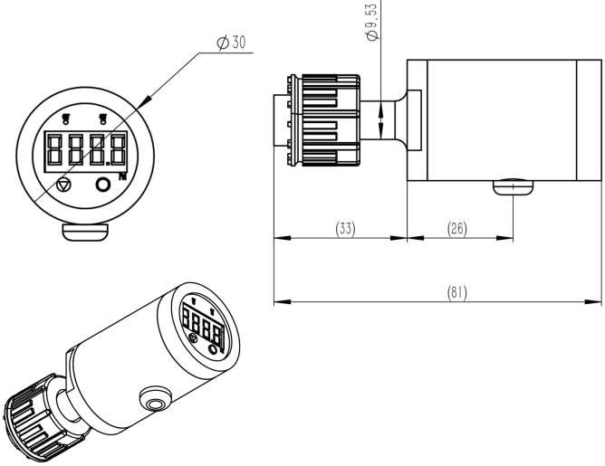
3/8" Pillar
